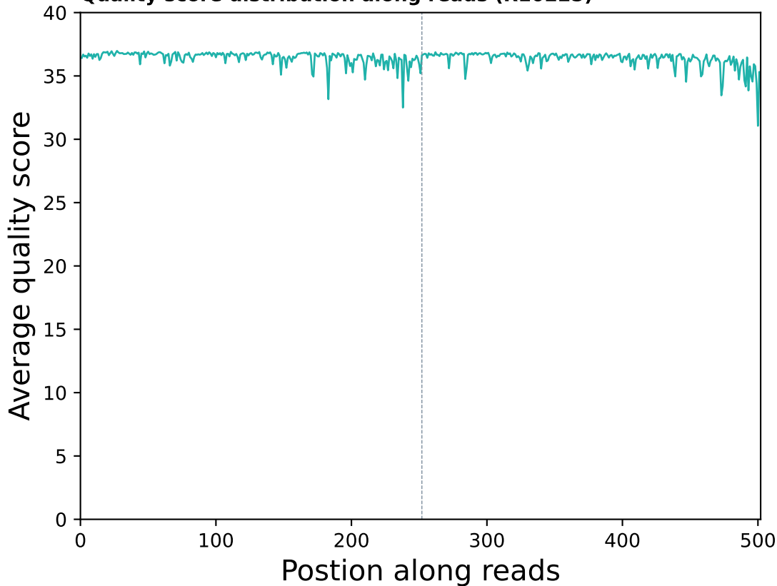
Quality score distribution along reads (R10225)
